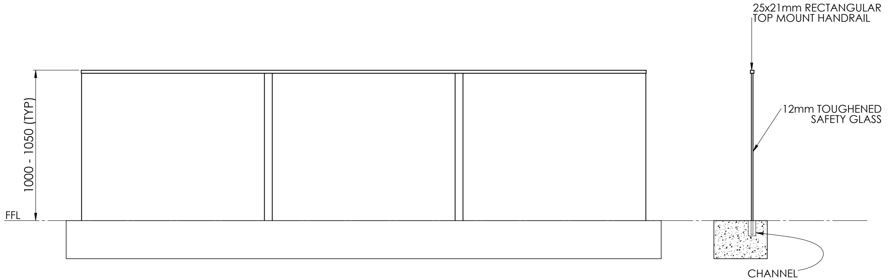
FRONT VIEW
