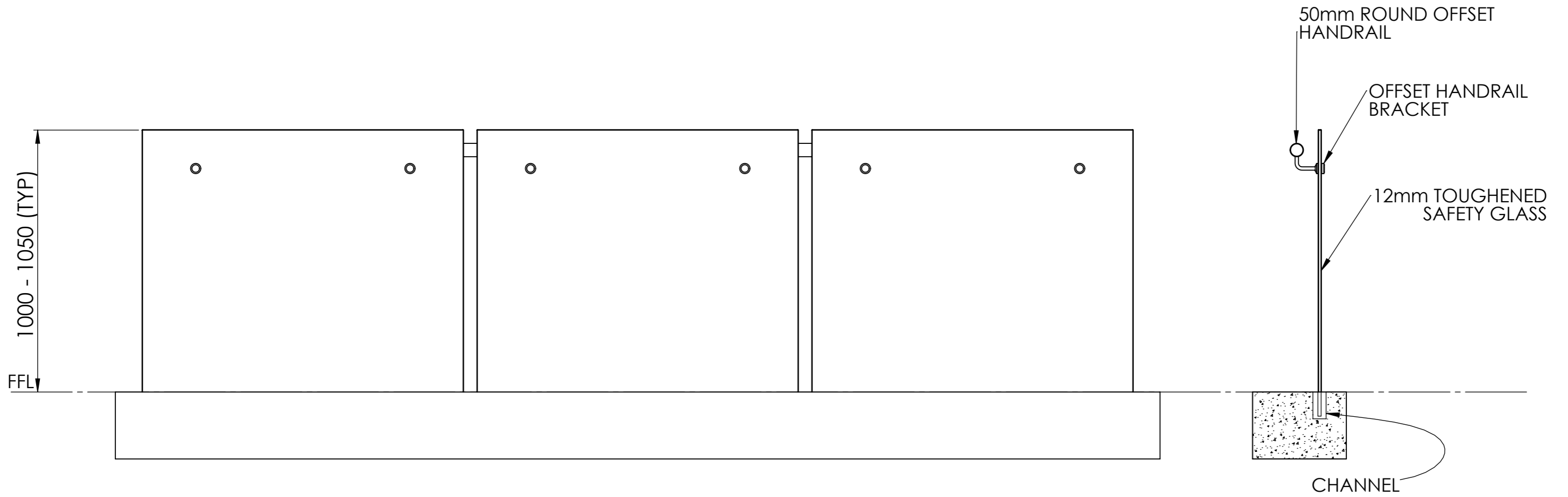
FRONT VIEW
