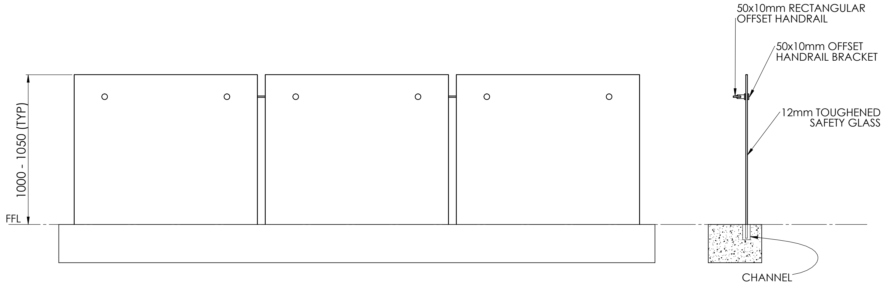
FRONT VIEW
