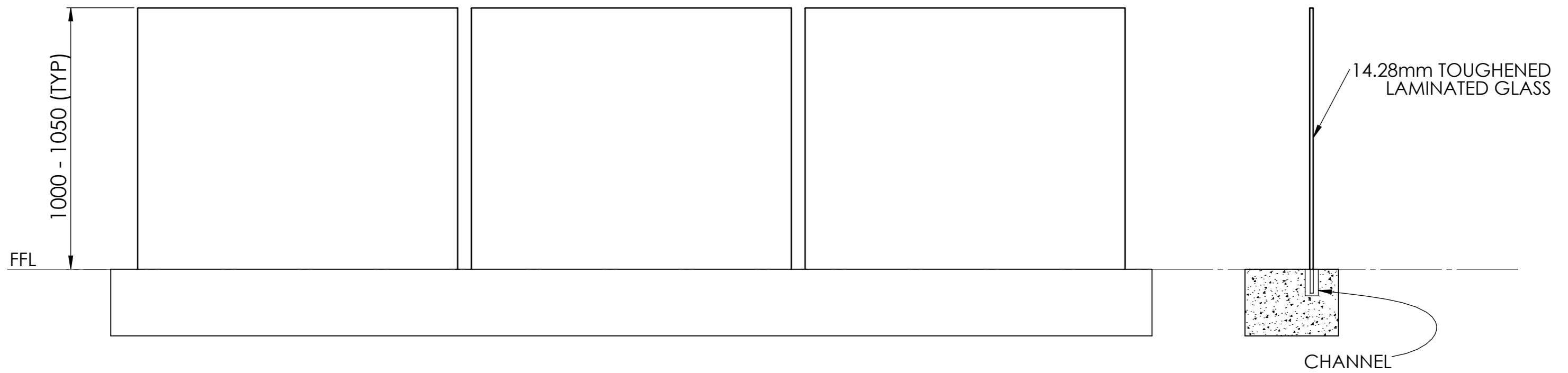
FRONT VIEW
