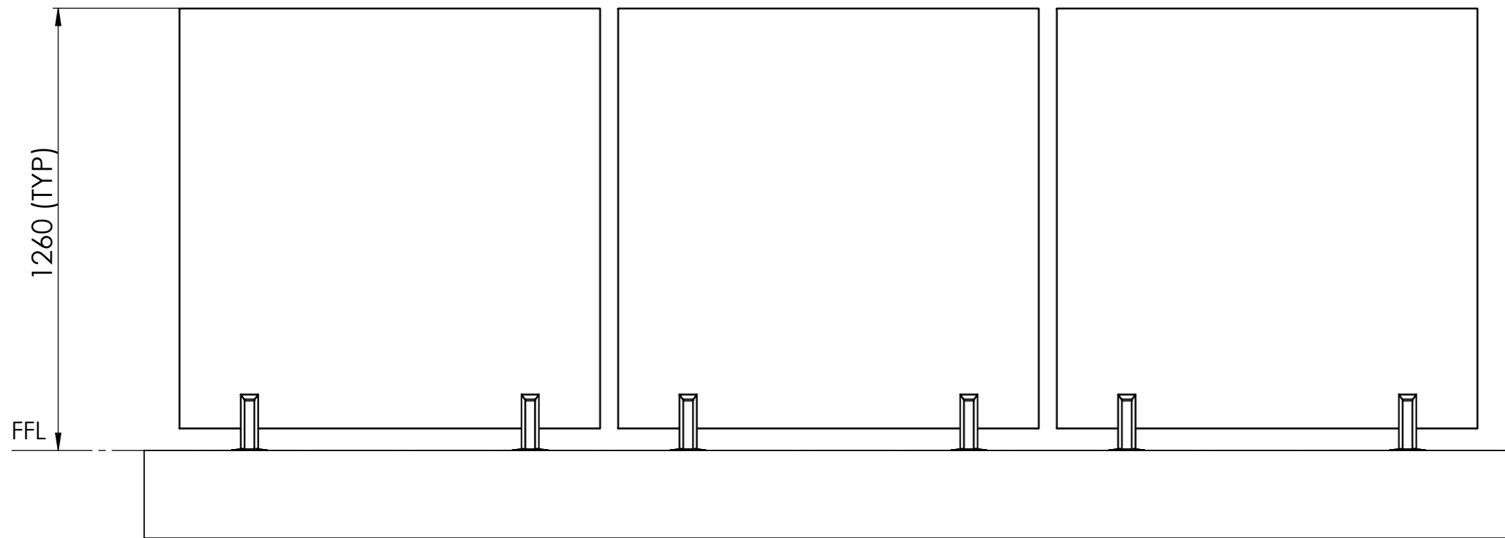
FRONT VIEW
