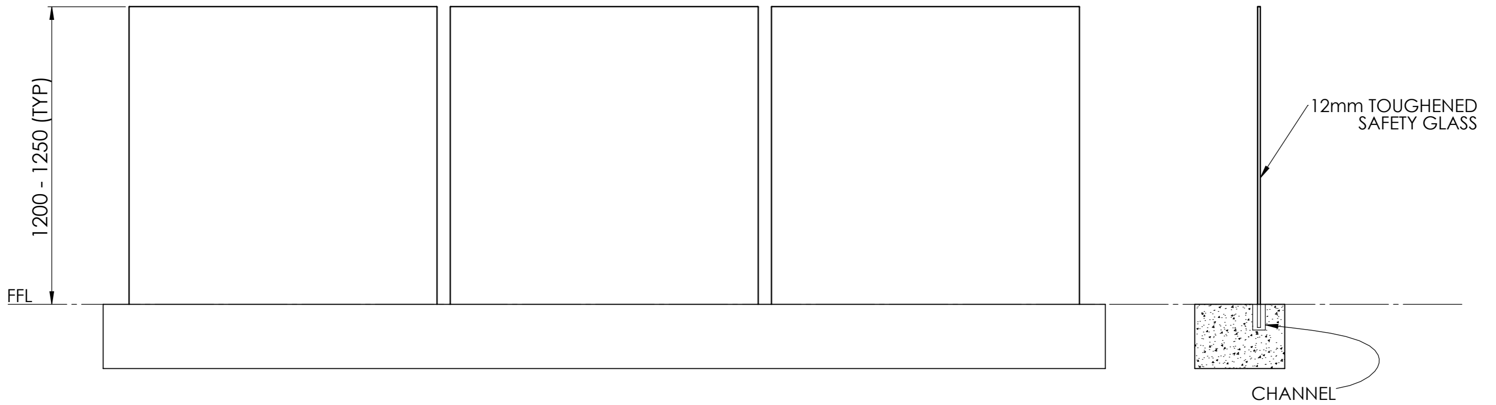
FRONT VIEW
