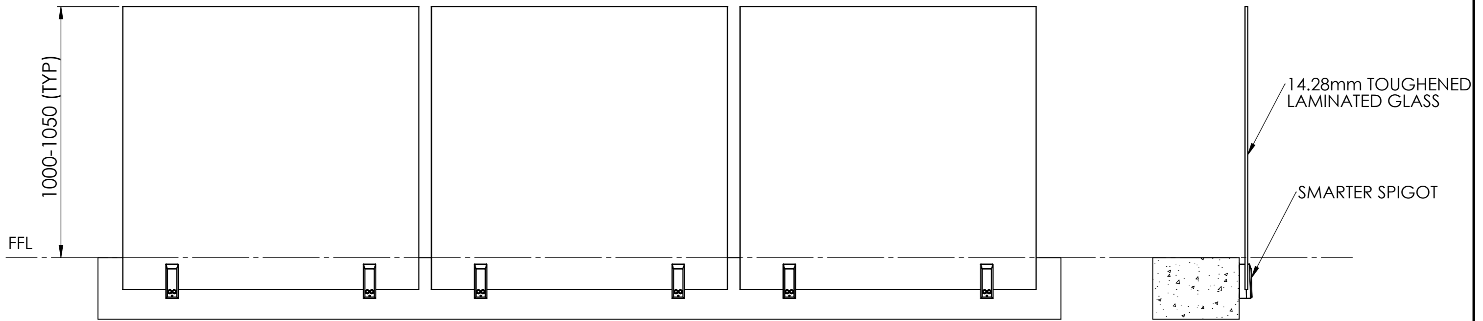
SECTION
