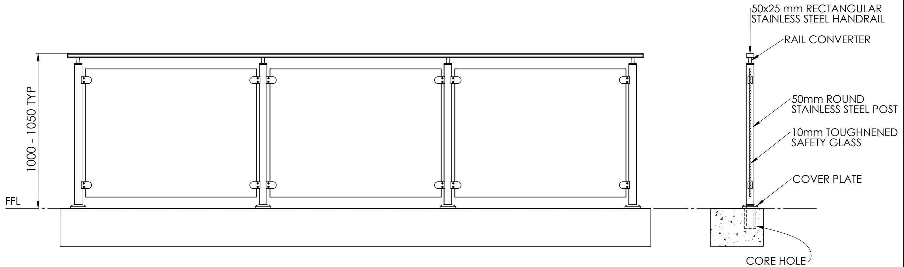
FRONT VIEW
